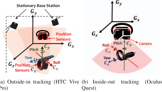
Fig. 4. Position tracking & coordinate systems in VR.
